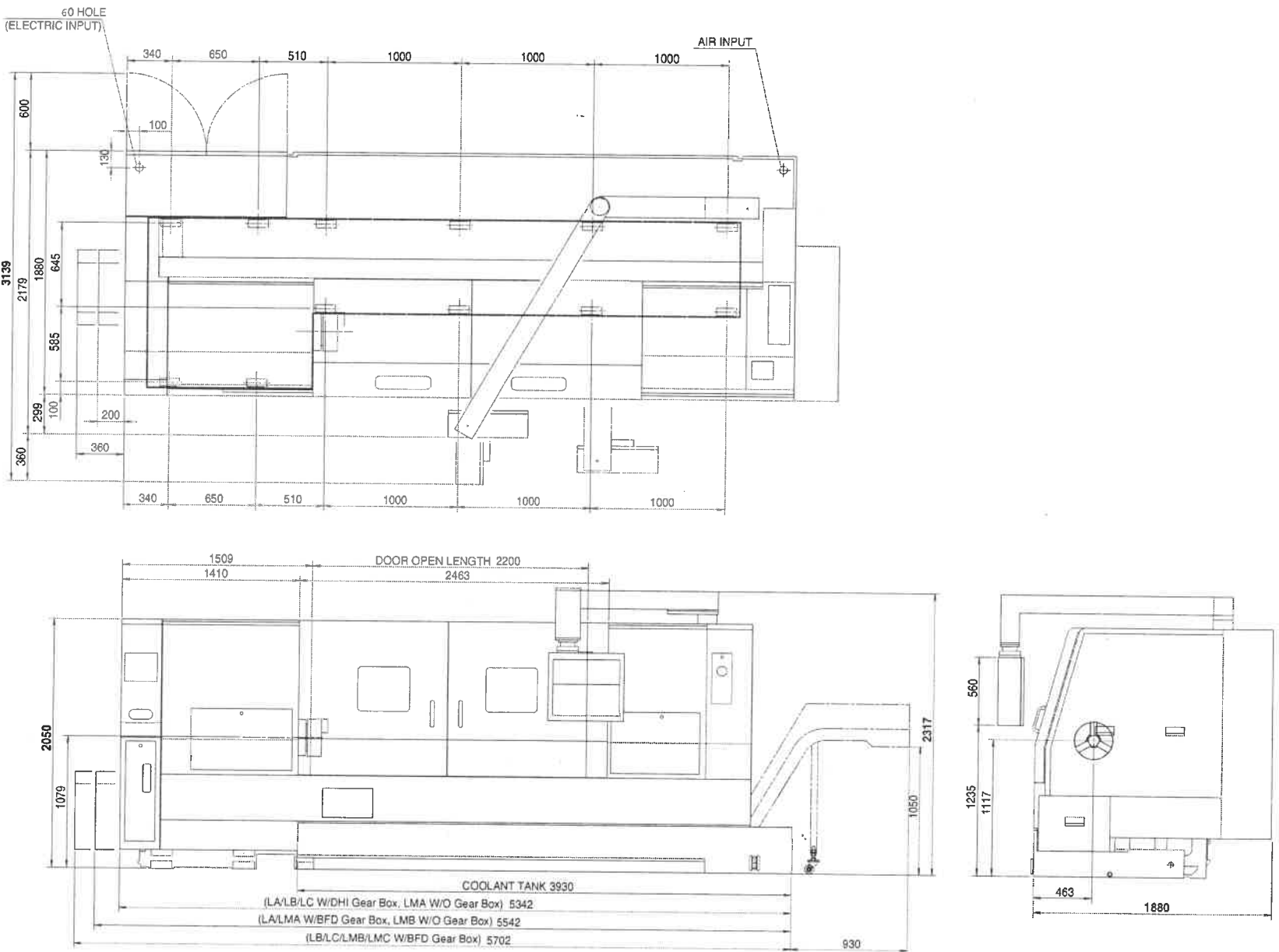
Fig. 3-2 Dimensional drawings
